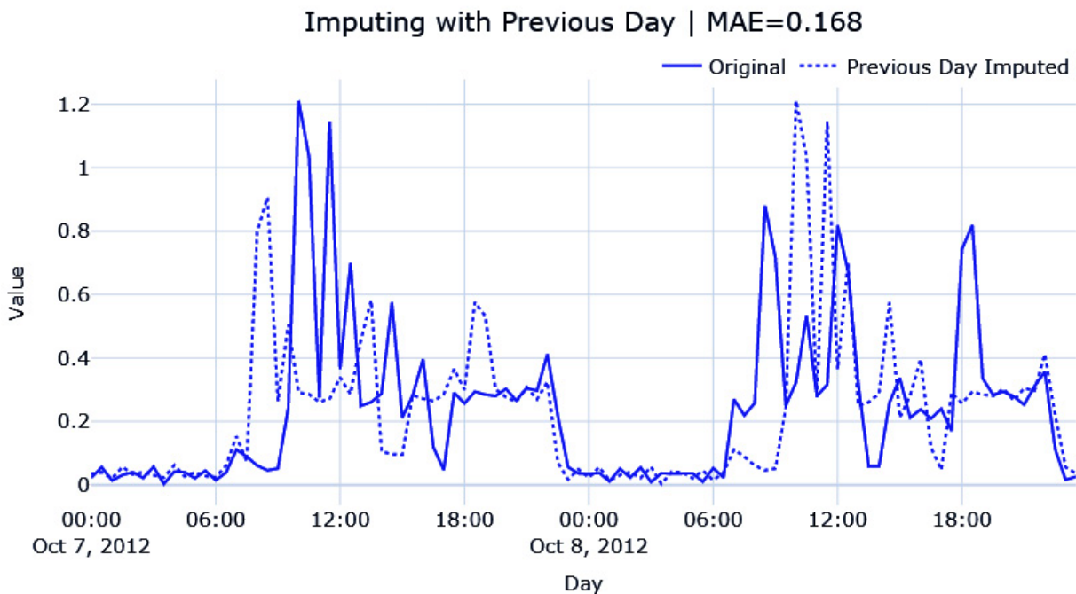
Figure 2.12 – Imputing with the previous day
