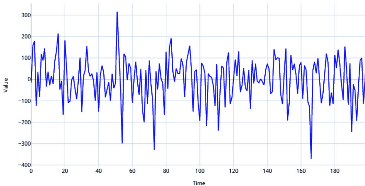
Figure 1.3 – White noise process
