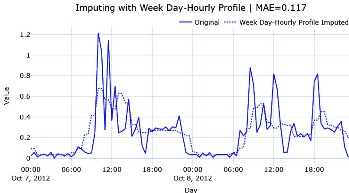
Figure 2.14 – Imputing the hourly average for each weekday
