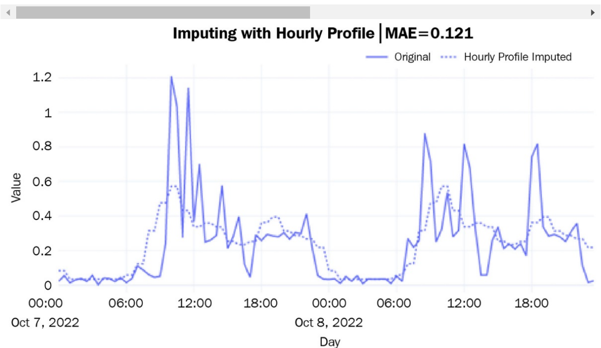
Figure 2.13 – Imputing with an hourly profile
