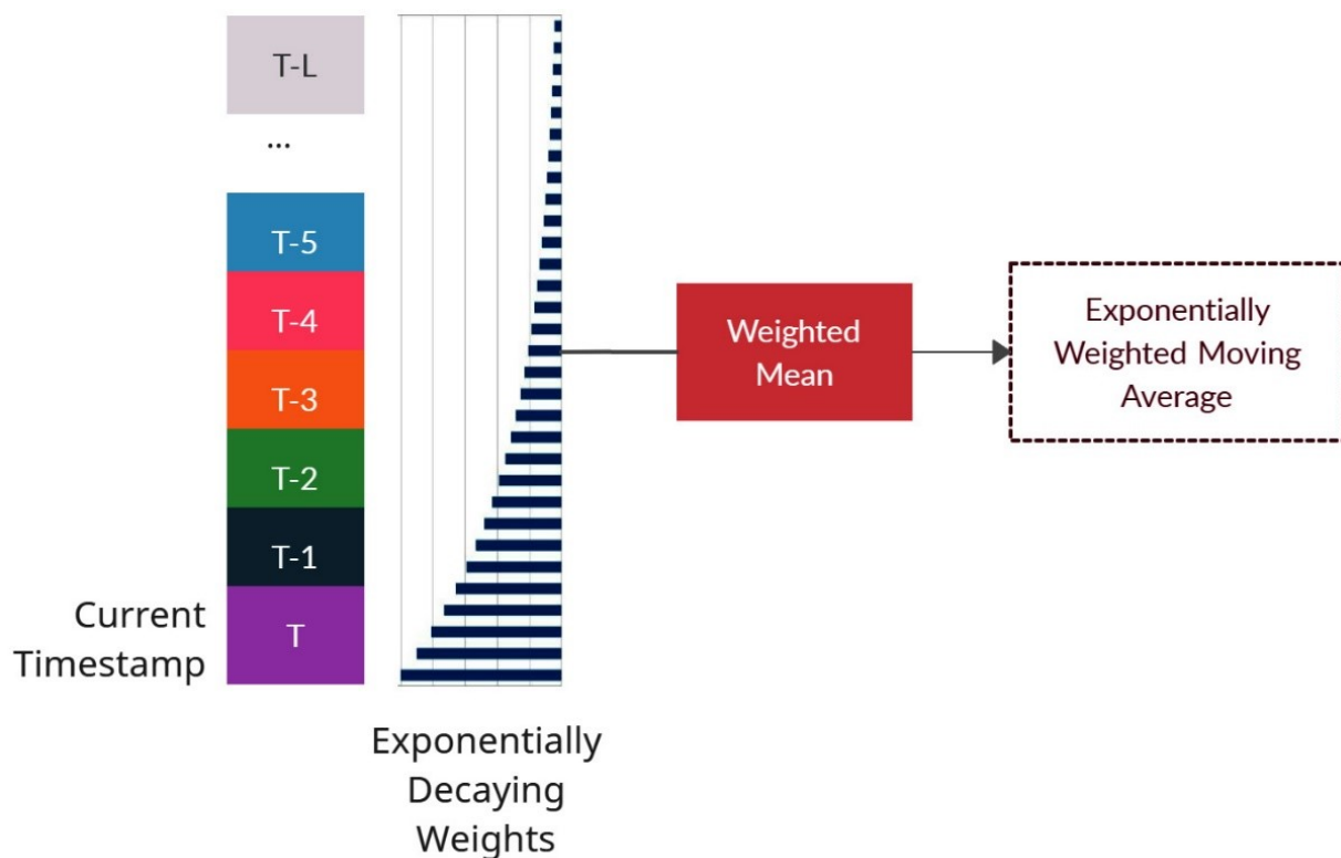
Figure 6.6 – EWMA features(Color figure)
