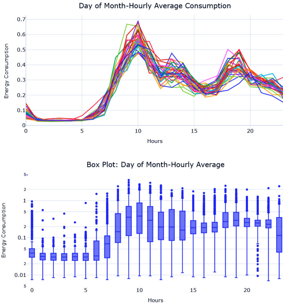
Figure 3.8 – Seasonal plot (top) and seasonal box plot (bottom) at an hourly resolution(Color Figure)
