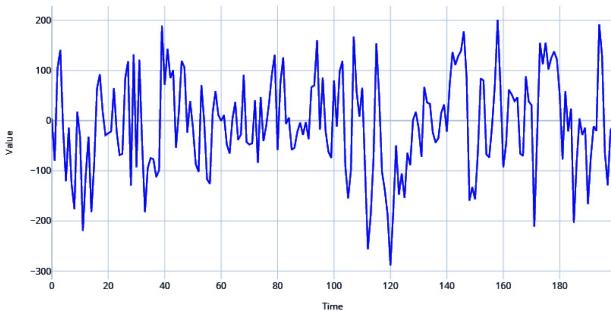
Figure 1.4 – Red noise process
