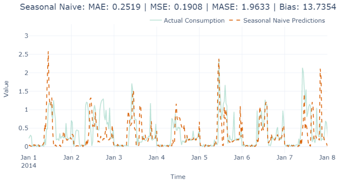
Figure 4.3 – Seasonal naïve forecast
