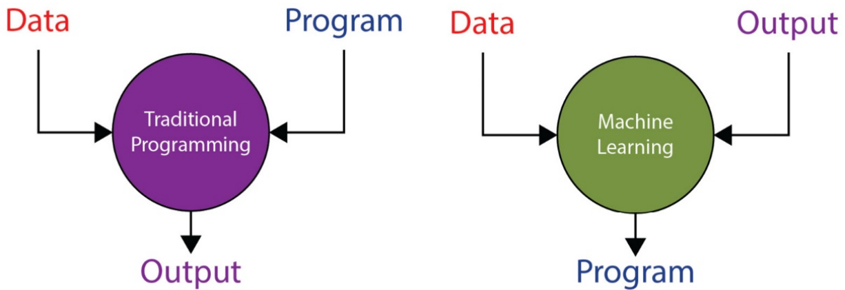
Figure 5.1 – Traditional programming versus machine learning
