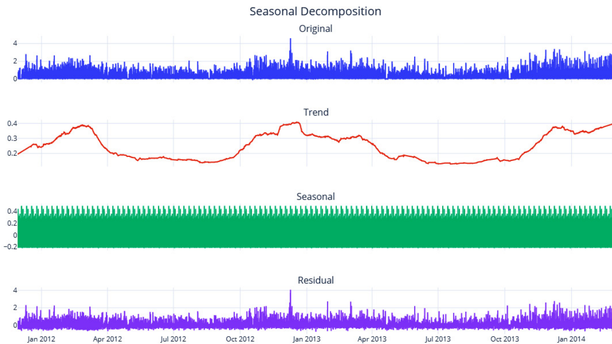
Figure 3.13 – Seasonal decomposition using statsmodels
