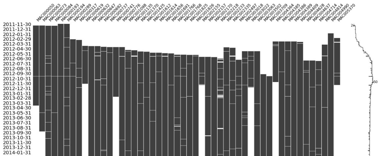
Figure 2.9 – Visualization of the missing data in block 7
