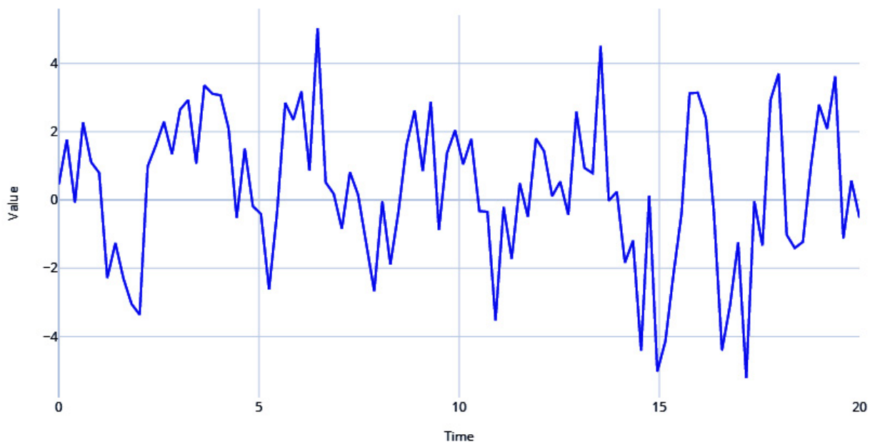
Figure 1.8 – Pseudo-periodic signal with AR and white noise
