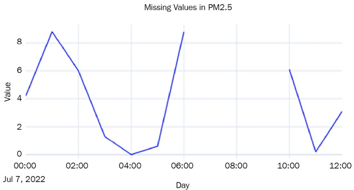
Figure 2.3 – Missing values in the Air Quality dataset
