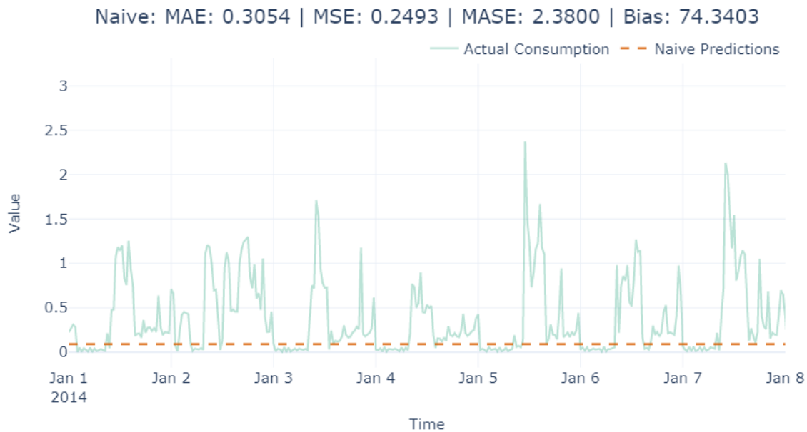
Figure 4.1 – Naïve forecast
