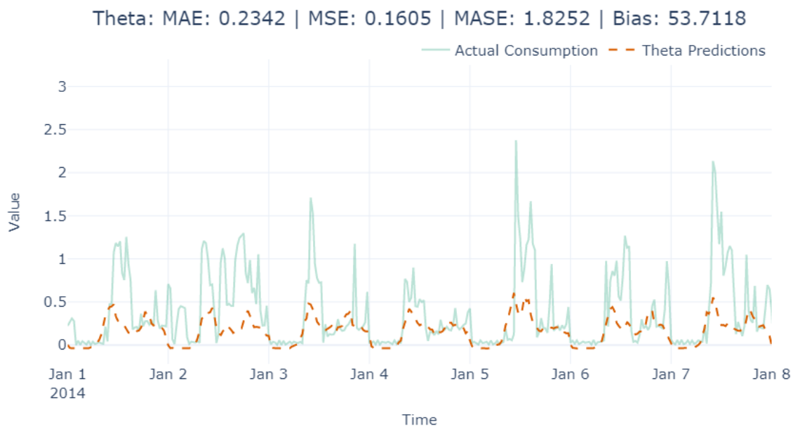
Figure 4.6 – The Theta Forecast
