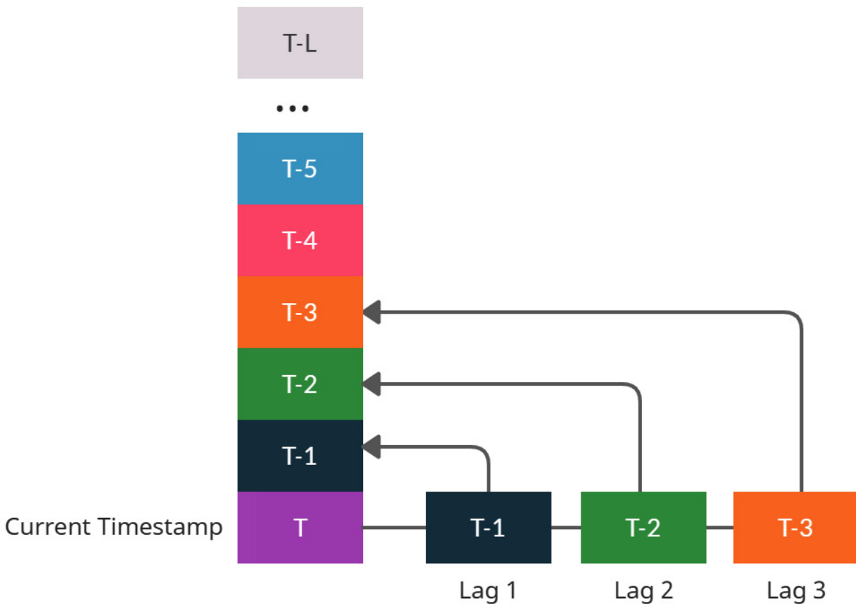
Figure 6.2 – Lag features (Color figure)
