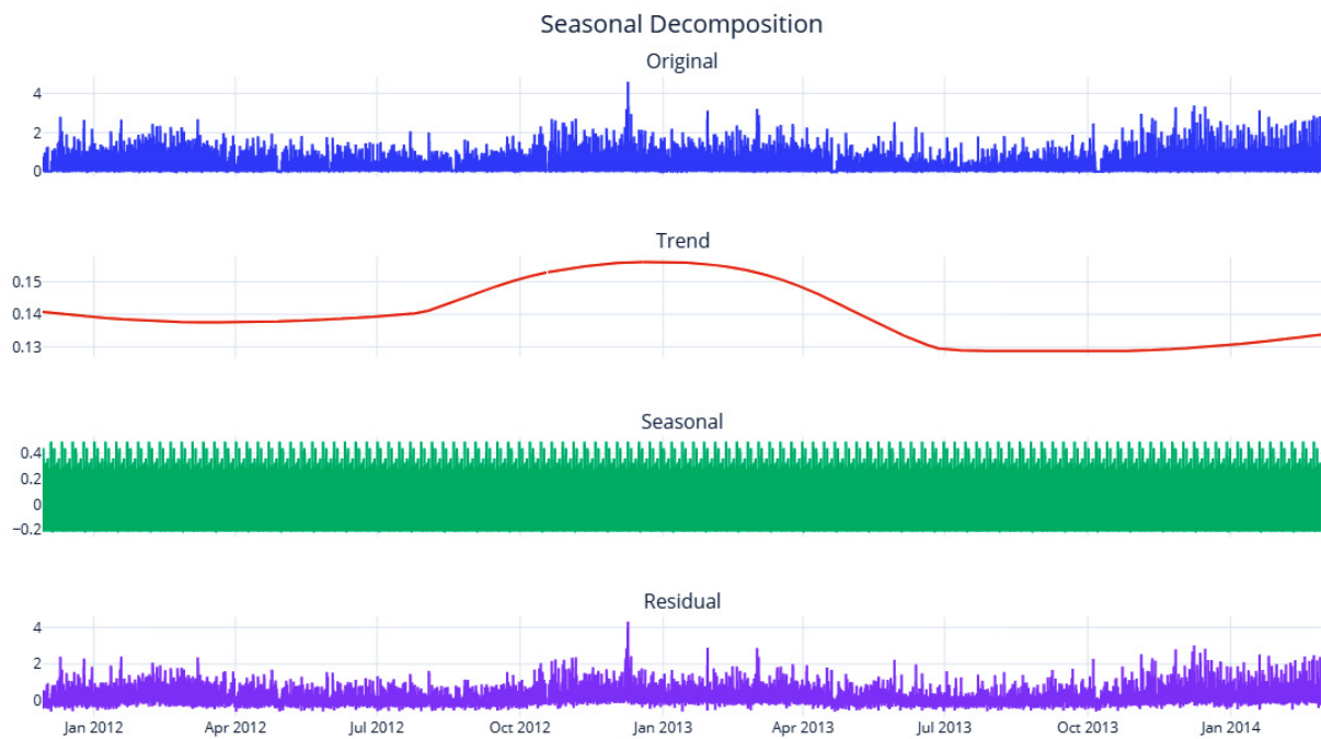
Figure 3.14 – STL decomposition
