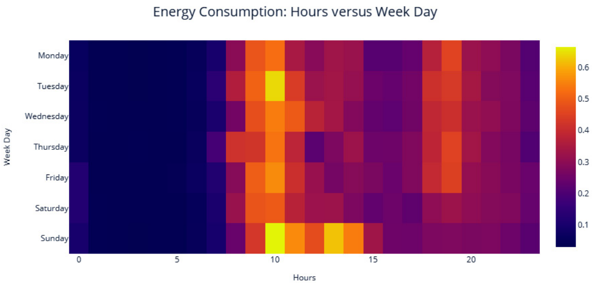
Figure 3.9 – A calendar heatmap for energy consumption(Color Figure)
