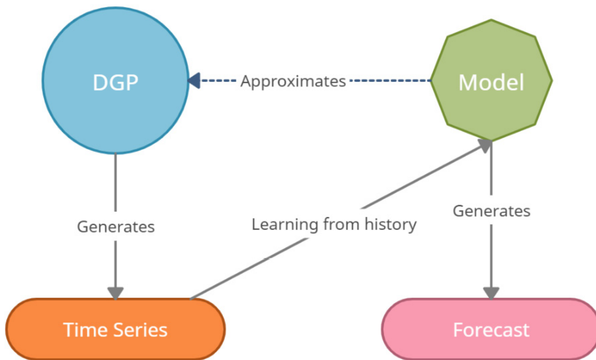
Figure 1.2 – DGP, model, and time series (Color)
