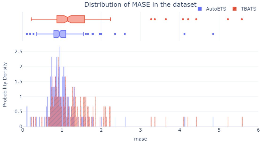
Figure 4.13 – The distribution of MASE and forecast bias of the baseline forecast in the validation dataset
