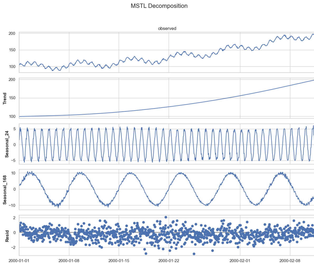
Figure 4.8 – Decomposed Time Series
