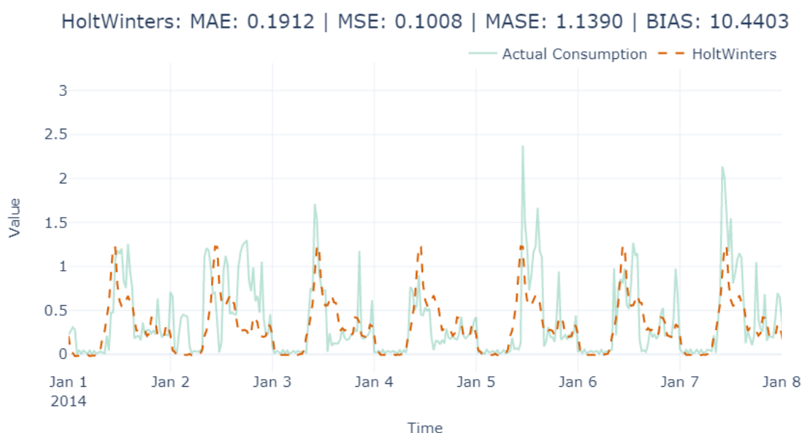
Figure 4.4 – Exponential smoothing forecast
