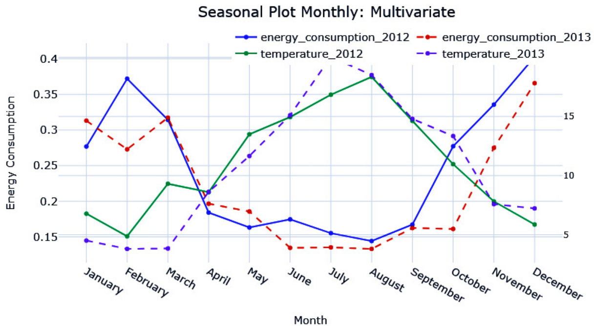
Figure 3.7 – Seasonal plot at a monthly resolution (energy consumption versus temperature) (Color Figure)
