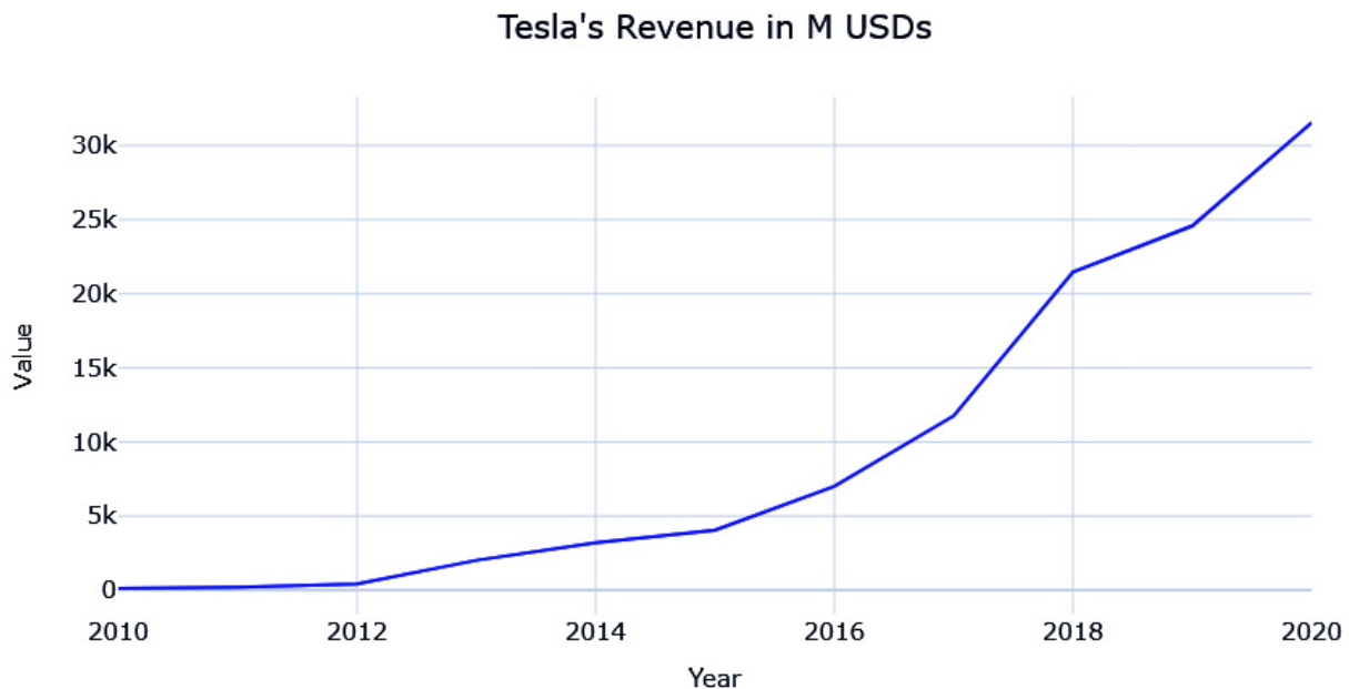
Figure 3.1 – Tesla's revenue in millions of USD
