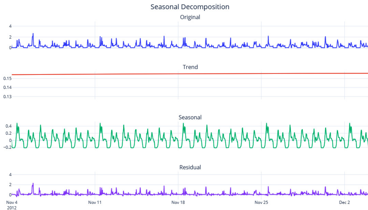
Figure 3.15 – STL decomposition (zoomed-in for a month)
