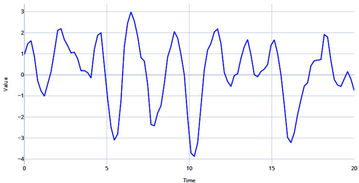
Figure 1.7 – AR signal
