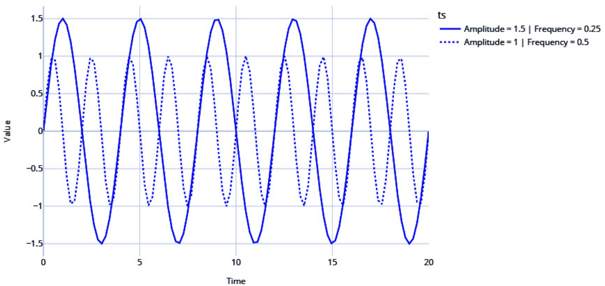
Figure 1.5 – Sinusoidal waves
