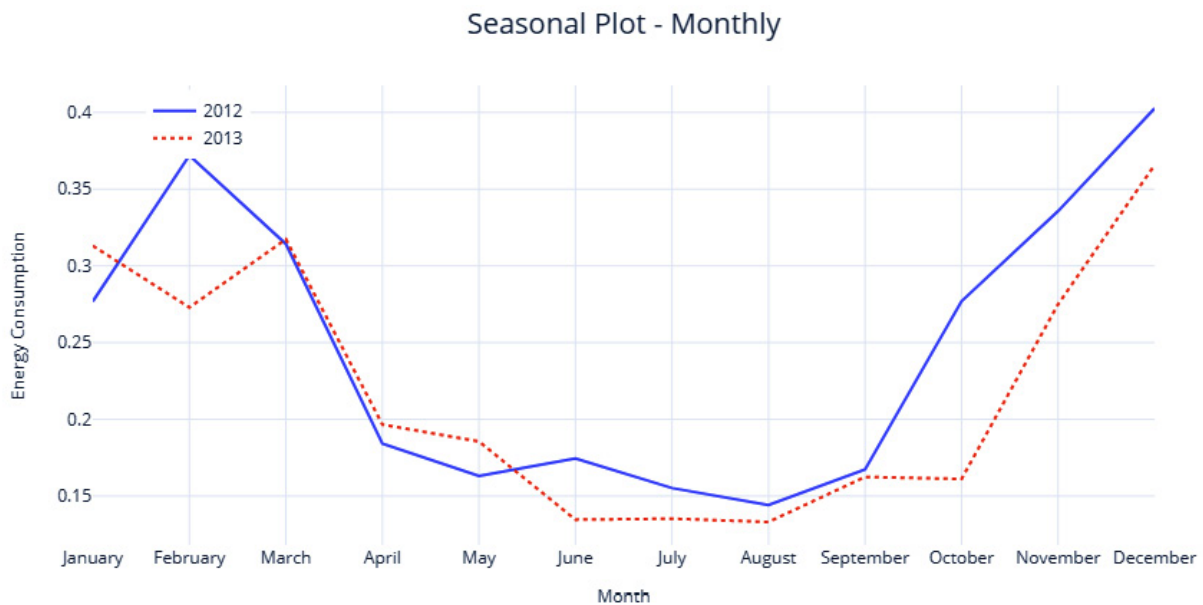
Figure 3.6 – Seasonal plot at a monthly resolution(Color Figure)
