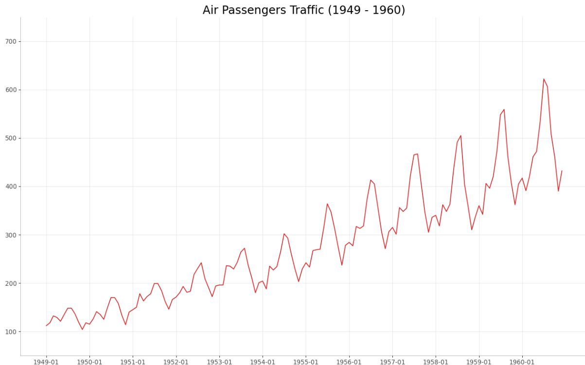
Figure 1.10 – Air Passengers Dataset – Example of Heteroscedastic Time Series
