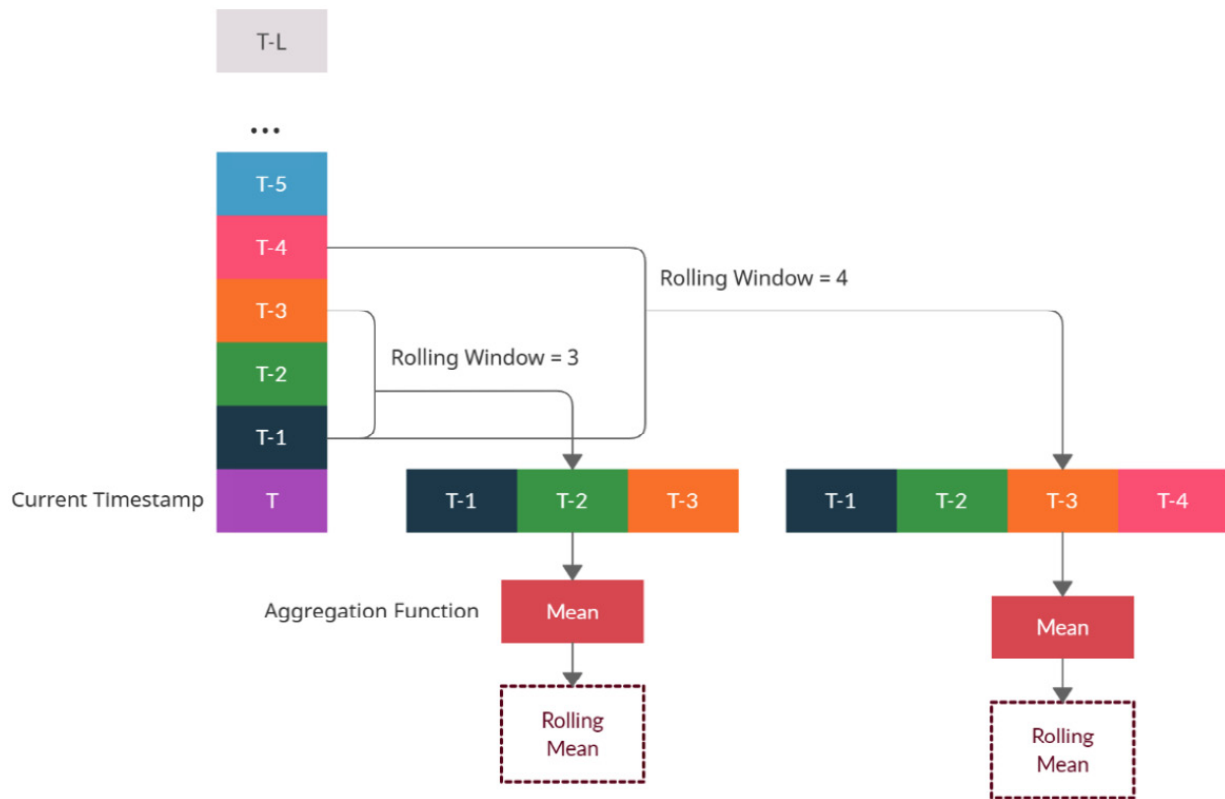
Figure 6.3 – Rolling window aggregation features(Color figure)
