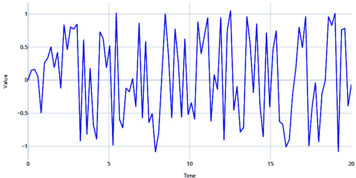
Figure 1.6 – Pseudo-periodic signal
