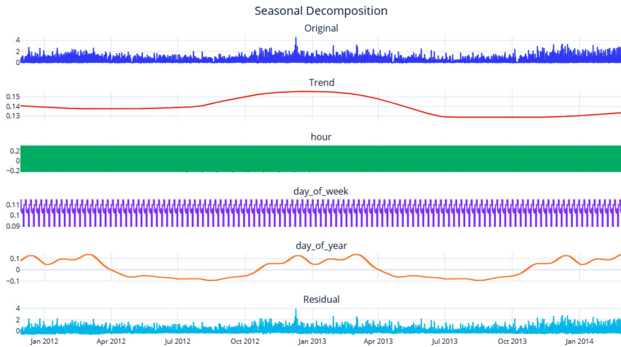
Figure 3.17 – Multiple seasonality decomposition using Fourier terms
