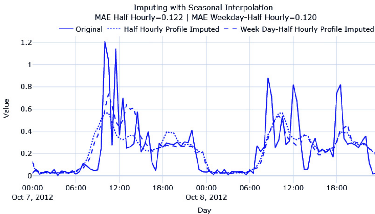
Figure 2.15 – Imputing with seasonal interpolation
