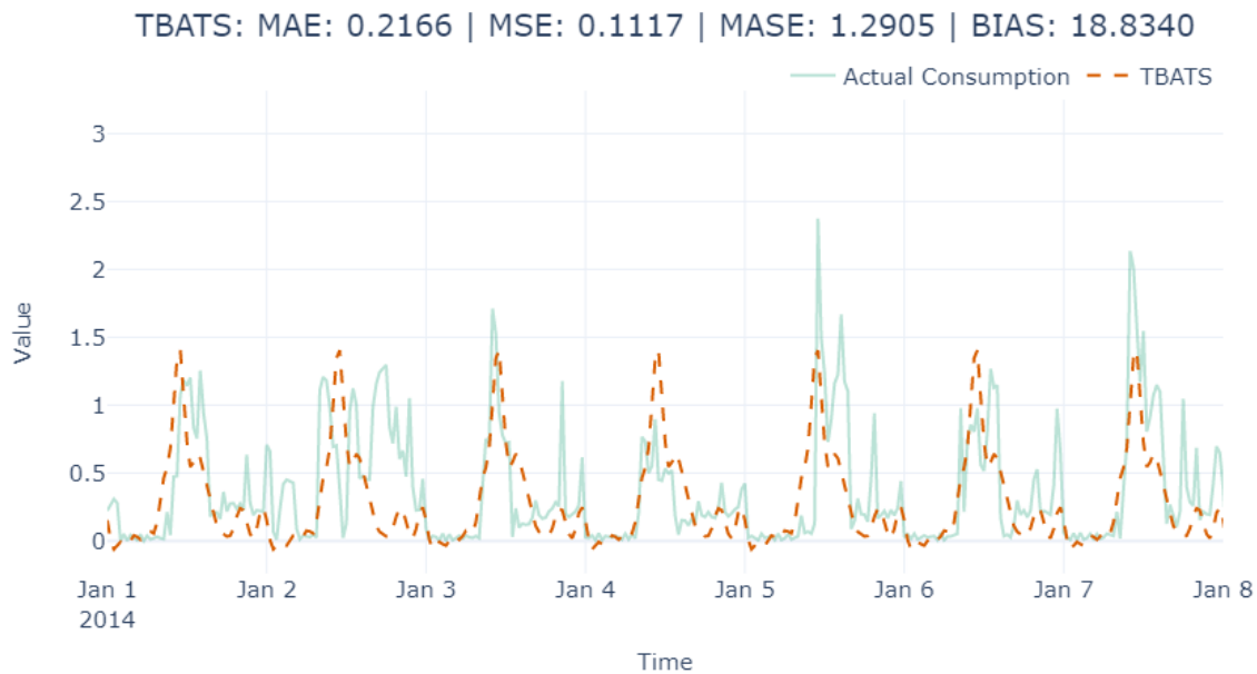
Figure 4.9 – TBATS forecast
