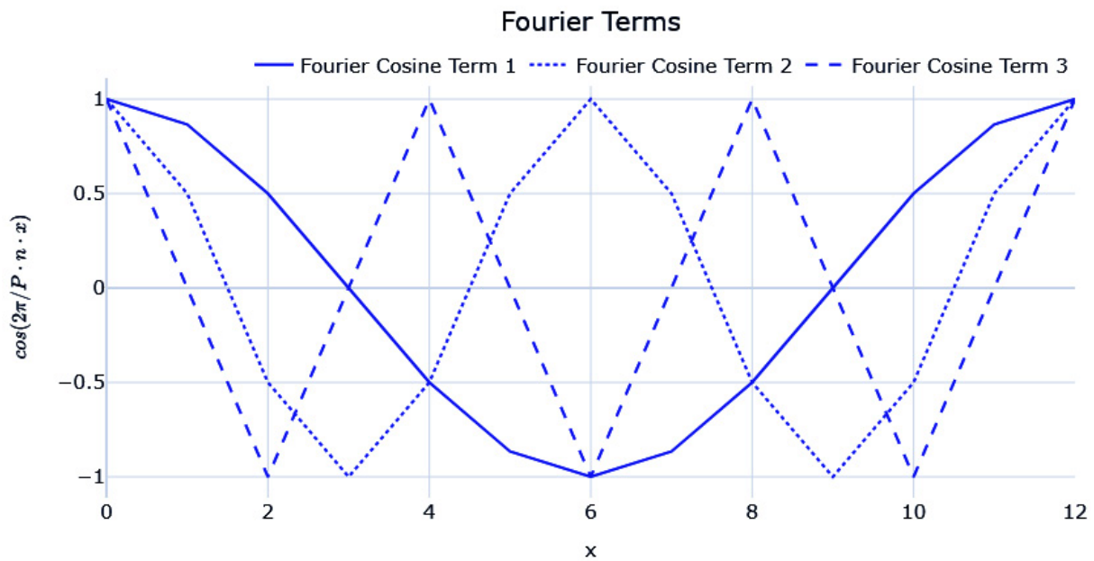
Figure 3.11 – Cosine Fourier terms ( n=1, 2, 3 )
