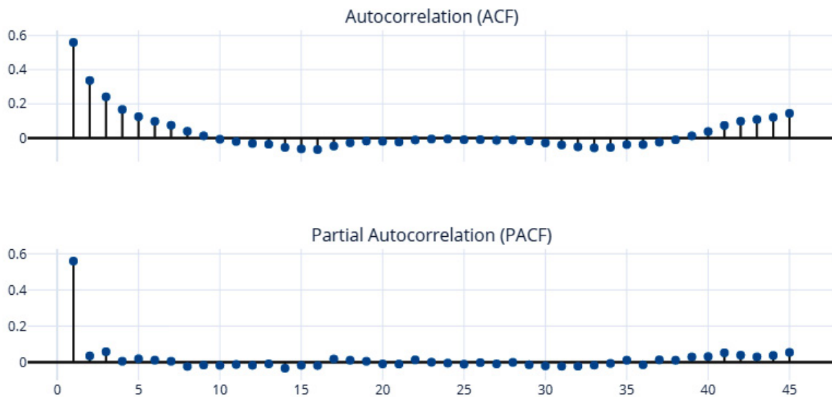
Figure 3.10 – Autocorrelation and partial autocorrelation plots
