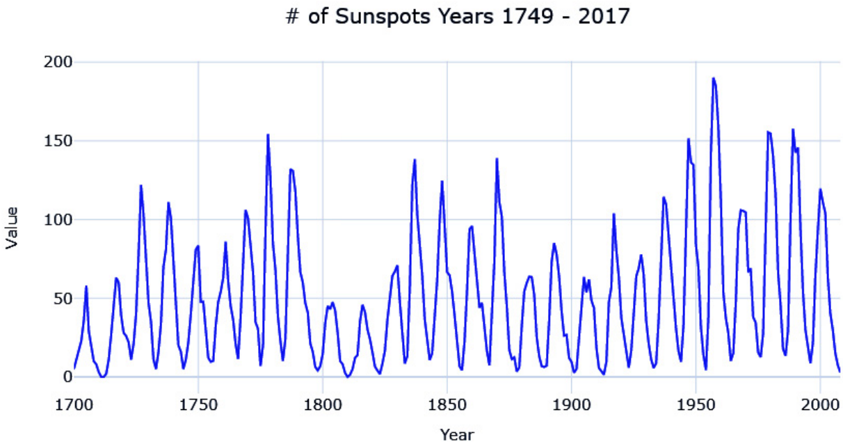
Figure 3.2 – Number of sunspots from 1749 to 2017
