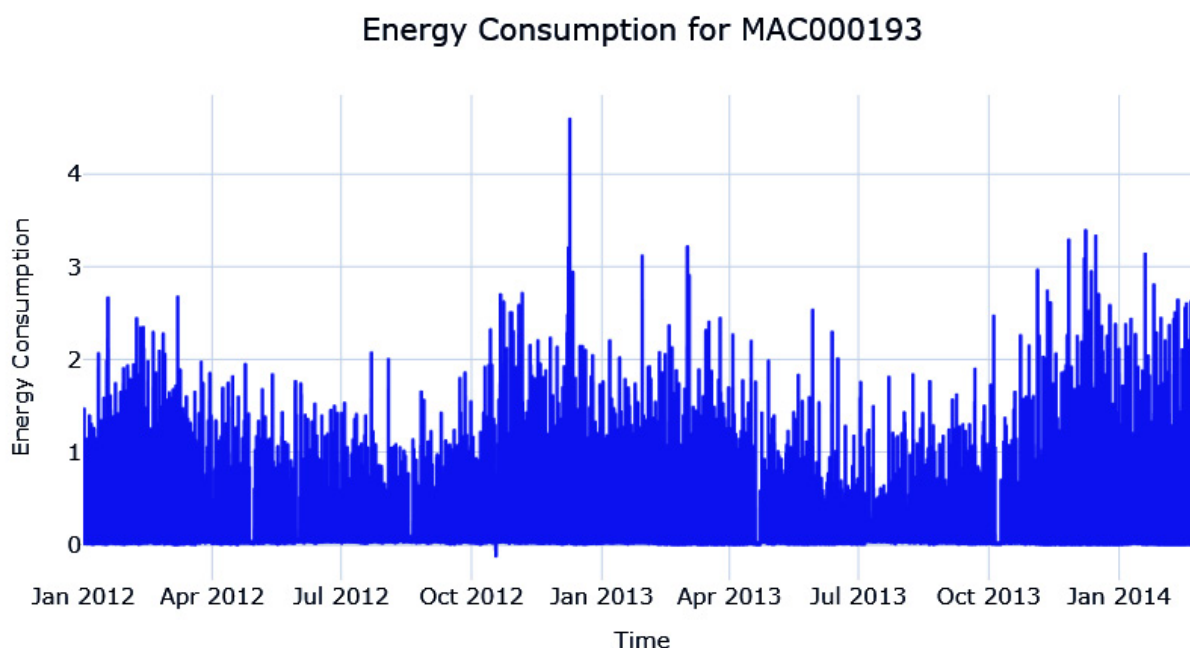
Figure 3.3 – Line plot of household MAC000193
