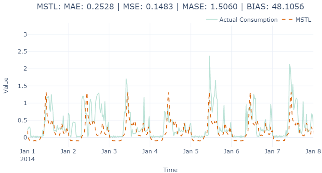
Figure 4.10 – MSTL forecast
