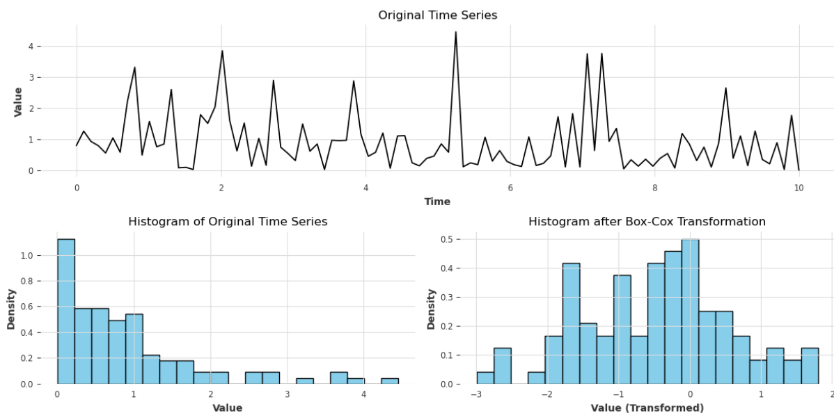
Figure 4.7 – Box-Cox Transformation
