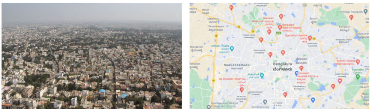
Figure 1.1 – An aerial view of Bengaluru (left) and a map of Bengaluru (right) (Color)
